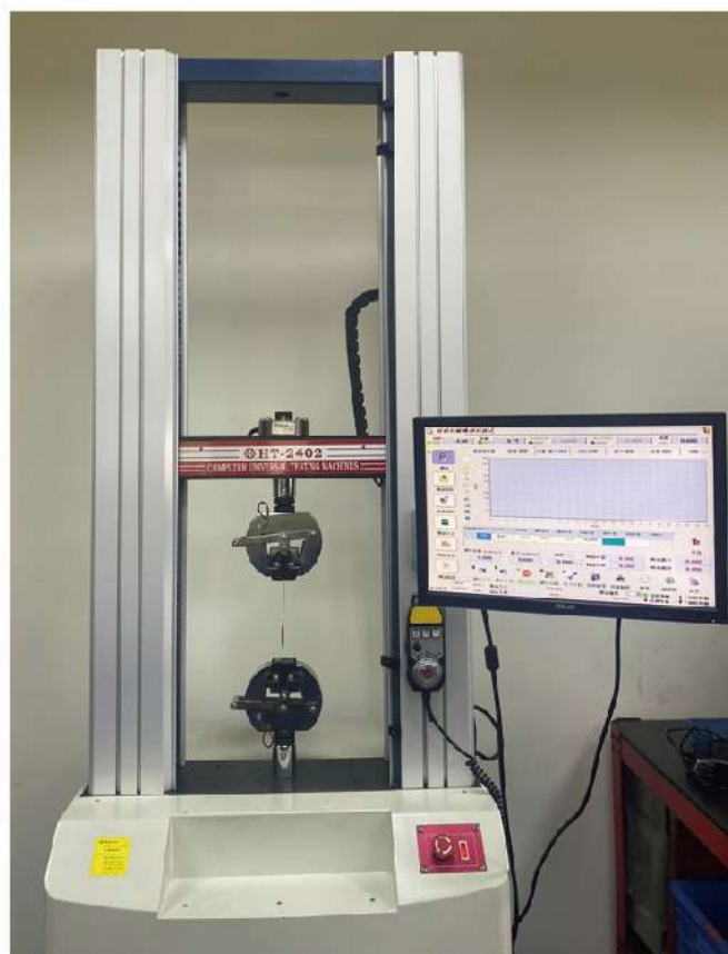
▲ Compression and tensile testing machine
