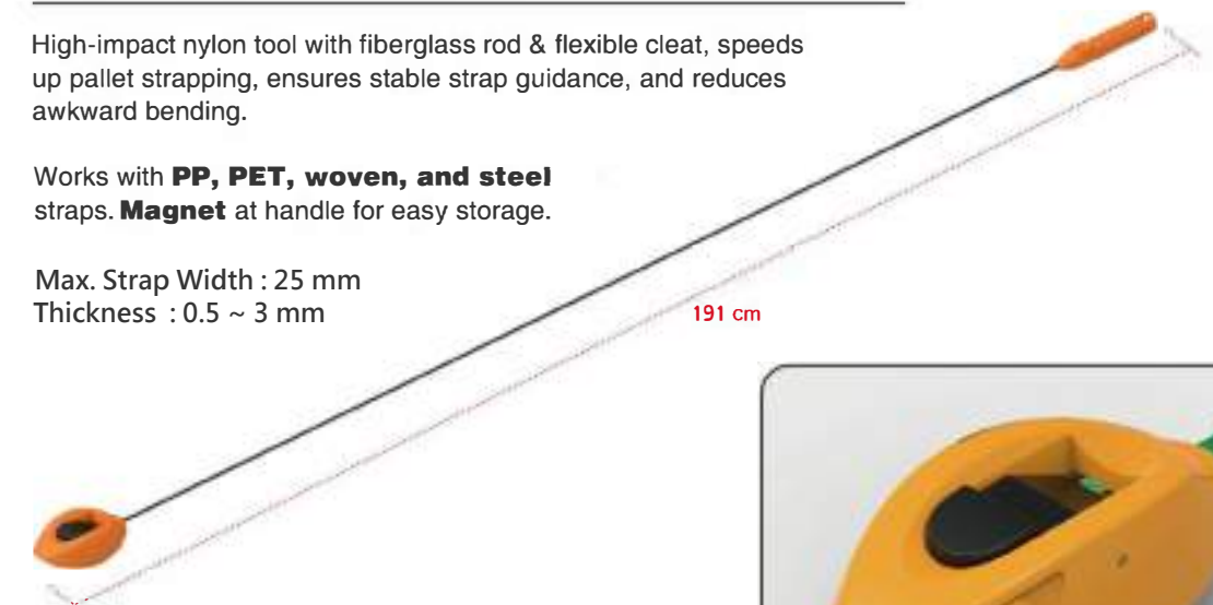
▶ LR403 Pallet Threading Tool
