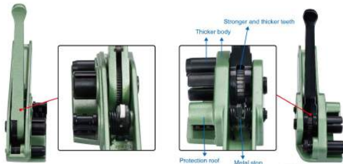
P270 Heavy Duty
